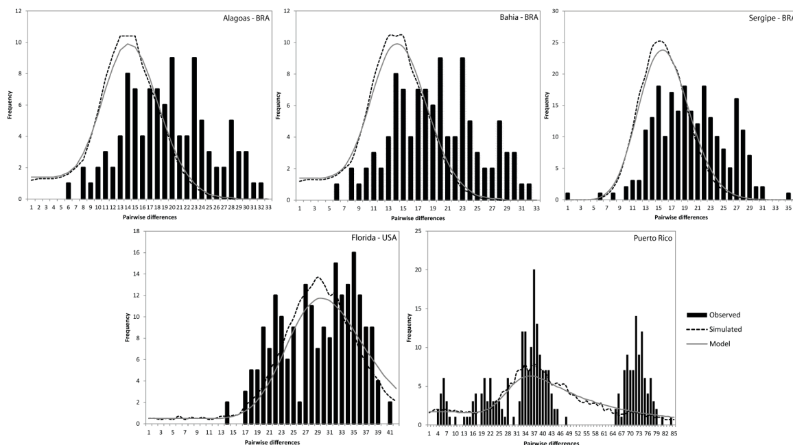
Figure 6. Frequency distributions of the number of pairwise nucleotide differences (mismatch) between C. guanhum i haplotypes for all populations.
