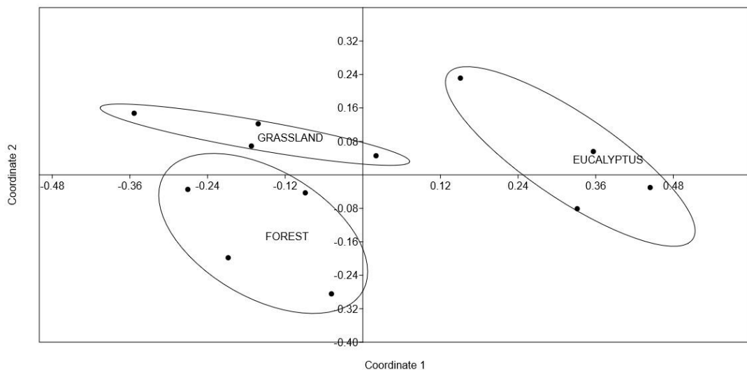
Figure 3.1. Non-metric multi-dimensional scaling plot of collembola assemblages sampled in three different land-use types (Forest, Grassland, Eucalyptus plantation) based on Bray-Curtis resemblance matrix calculated using abundance data.
