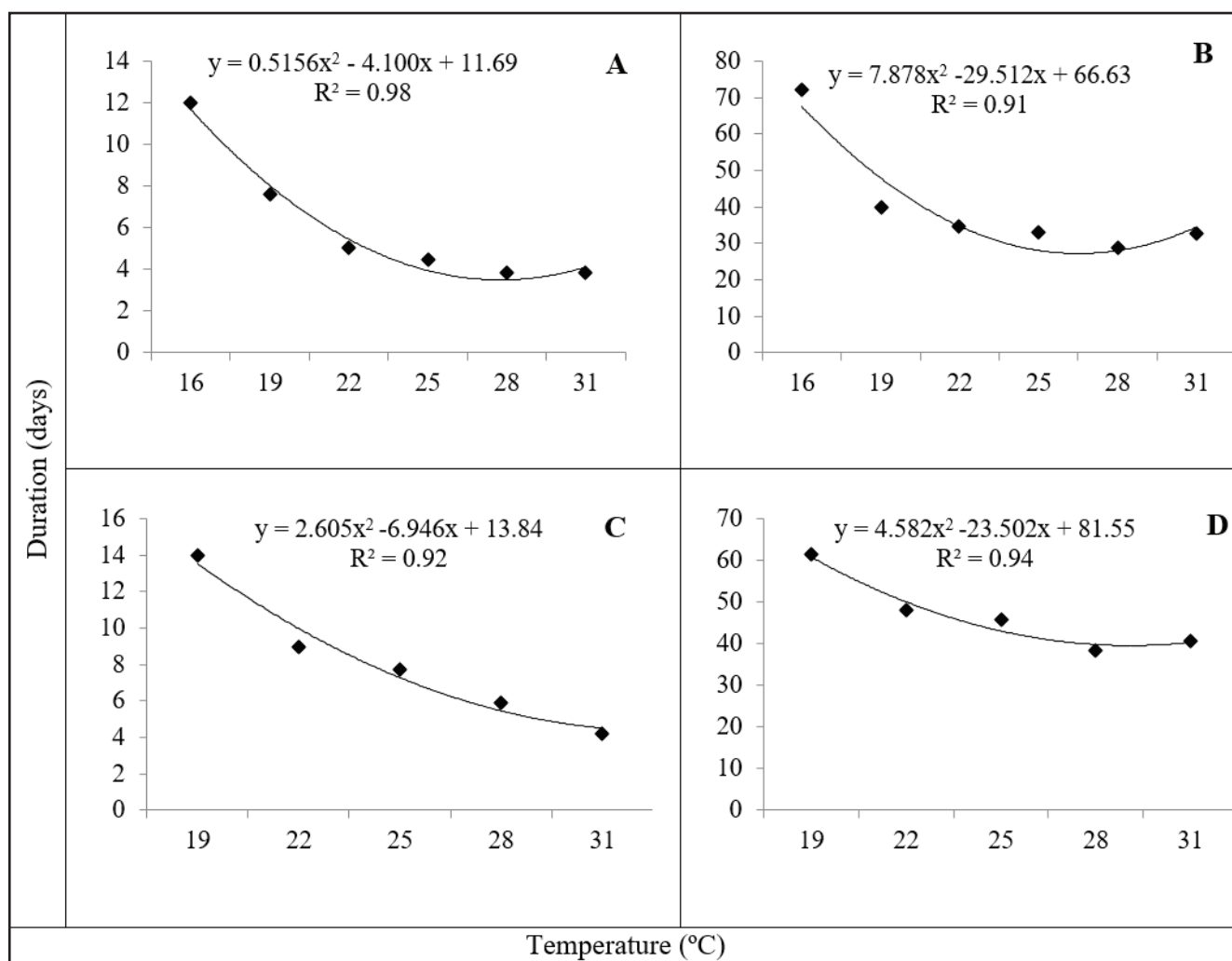
Figure 1. Regression curves adjusted for the duration of egg (A), larvae (B), pupae (C) and biological cycle (egg-adult) periods of Lobiopa insularis under different temperatures ( 70\pm 10\% RH; 12 h photophase).
