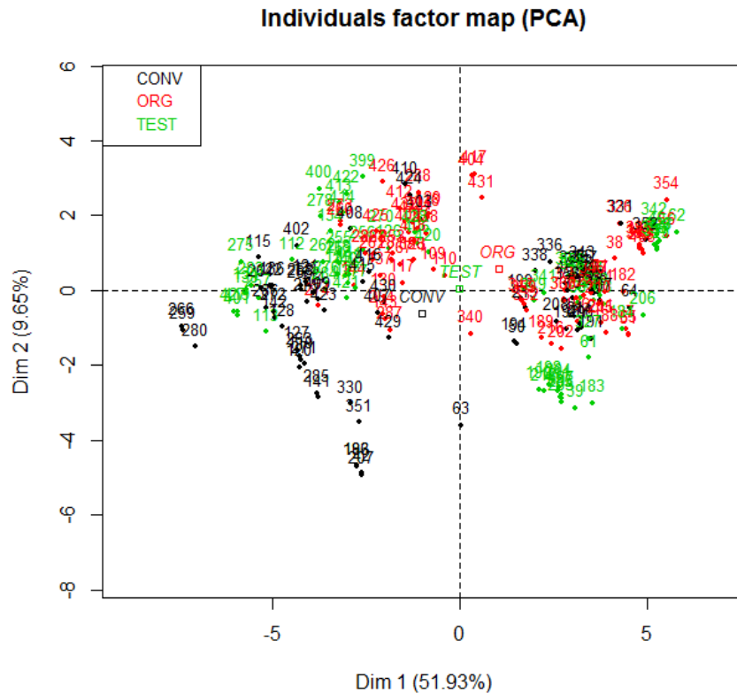
Figure 8: Dispersion of the PCA factors 1 and 2 scores of the samples under conventional fertilization (CONV), organic (ORG) and control (TEST) management, in a system without green manuring.
