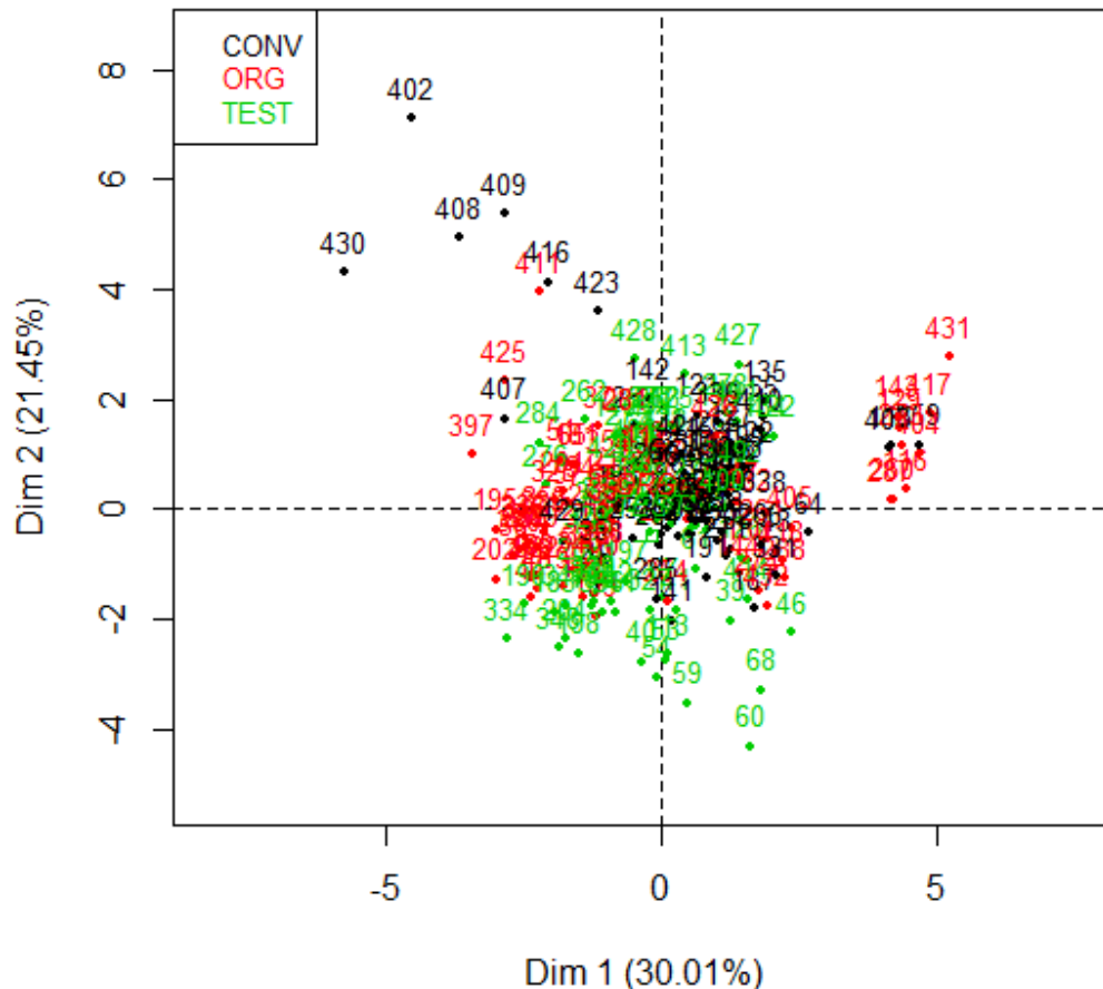
Figure 4: Dispersion of the PCA factors 1 and 2 scores of the samples under conventional fertilization (CONV), organic (ORG) and control (TEST) management, in a system without green manuring.
