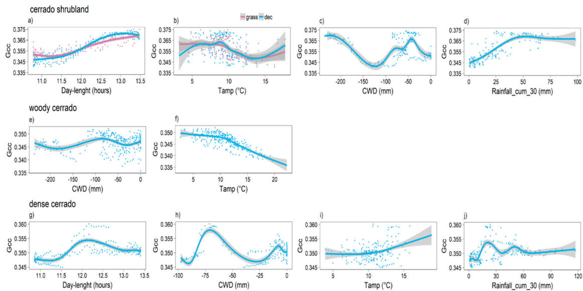
Figure 6. Response of the GAMMs fitted for the three-day 90th percentile values of the G_{cc} time series for deciduous leaf strategies (blue line) and grass (pink line) in the cerrado shrubland (a–d), woody cerrado (e,f), and dense cerrado (g–j) in relation to the following environmental variables: day-length, rainfall_lag7, Rainfall_cum_30, cwd , and Tamp .
