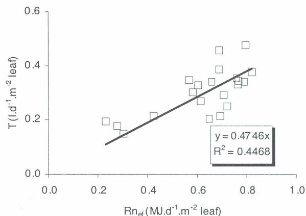
Figure 4. Relationship between transpiration ( T ) and effective net radiation ( Rn_{ef} ) for the whole coffee canopy.
