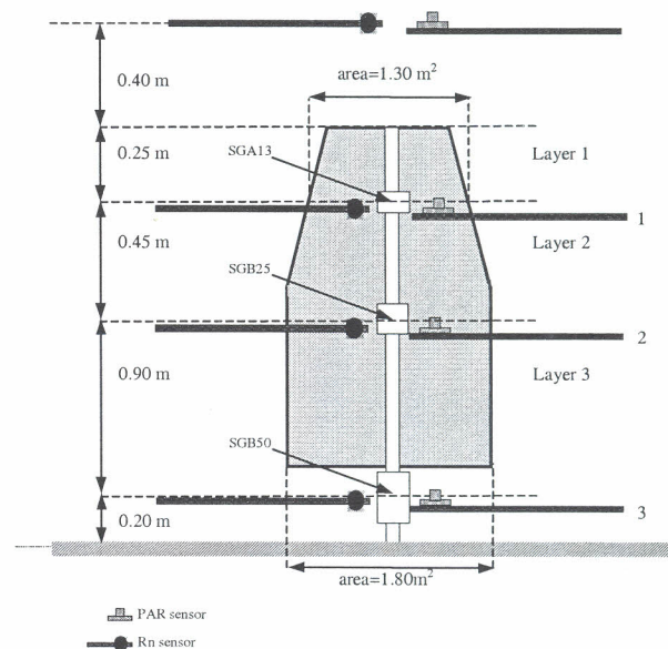
Figure 1. Schematic representation of the coffee plant studied and sensors location: sap flow sensors (SGB50, SGB25 e SGA13), Rn and PAR sensors, at positions 1, 2 and 3.
