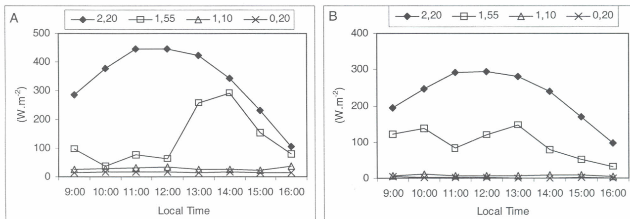
Figure 2. Average day-time fluctuation of: Rn (A), and PAR (B), measured above the canopy (2.2 m above the ground), and within the coffee canopy, at 1.55 m (bottom of L_1 ), at 1.10 m (bottom of L_2 ) and at 0.20 m (bottom of L_3 ).
