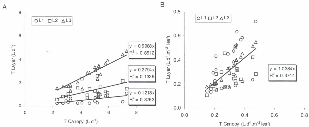
Figure 5. Relationship between the coffee canopy transpiration ( T_{\text{canopy}} ) and the transpiration at three layers of the coffee canopy ( T_{\text{layer}} ): A. transpiration on a volume basis; B. transpiration on a leaf area basis.
