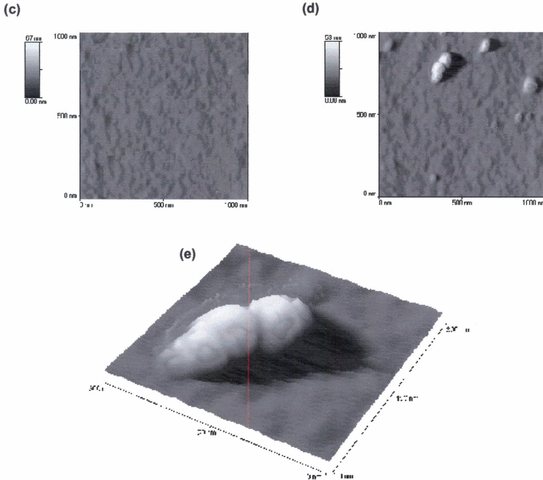
Figure 3 - AFM aspects of the scanned surfaces where changes in topographical features can be observed: in (a) as-hydrophilic fiber, (b) 5-min surfactant immersion (c) 10-min immersion and (d) 12-min immersion. Ridges observed after 12-min indicate excess of deposited protein, as zoomed in (e).
