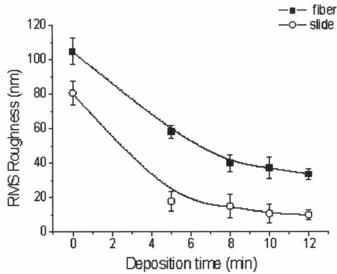
Figure 2 - RMS roughness as a function of deposition time.
