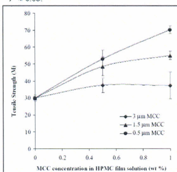
Figure 1: Tensile strength of HPMC films with different concentration and size of MCC
