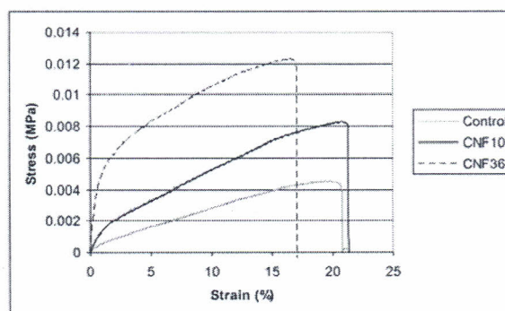
Figure 1: Stress-strain curves for MPEF with CNF loadings of 0% (control), 10% (CNF10), 36% (CNF 36).
