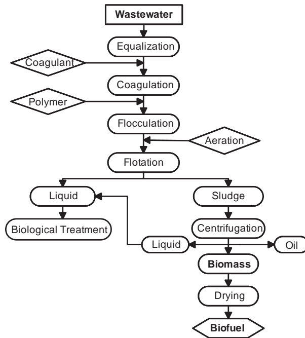
Figure 1. Processes involved in the wastewater treatment plant and obtention of biofuel (de Sena et al., 2008)
