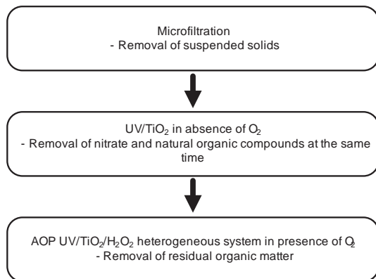
Figure 2. Process proposed for the treatment of secondary wastewaters with high concentration of nitrate/nitrite and recalcitrant organic compounds.
