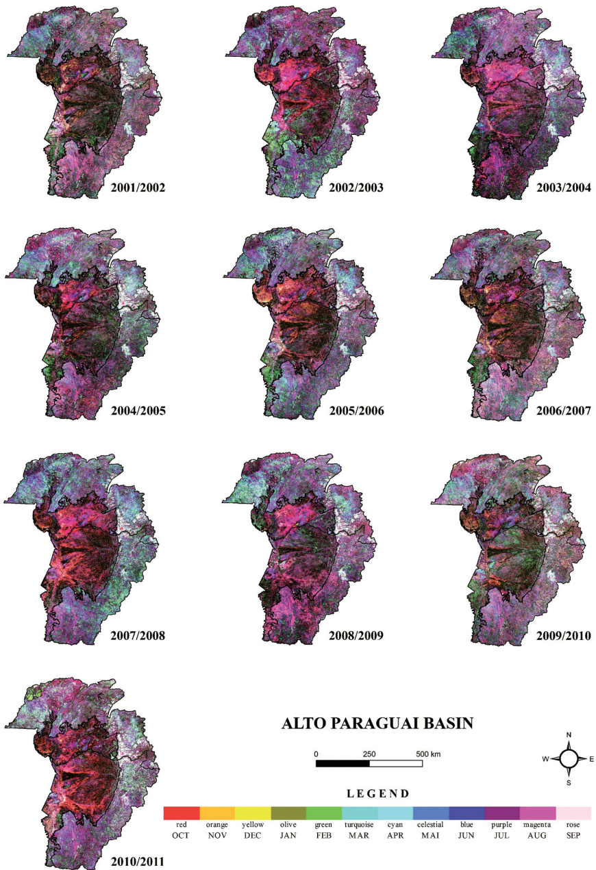
Figure 4 - HLS representation of BAP landscape for the 10 hydrologic years of the period from October 2001 to September 2011
