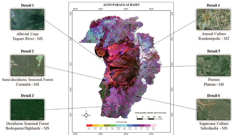
Figure 6 - HLS representation of BAP landscape for the period from October 2001 to September 2011
