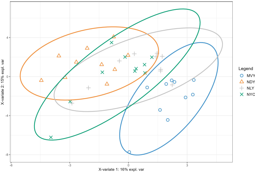
FIGURE 1 Partial least squares discriminant analysis (PLS-DA) score plot of serum metabolite distribution according to treatment. MVY, monensin + virginiamycin + live yeast; NLY, narasin + live yeast; NYC, narasin + yeast culture; NDY, narasin + active dry yeast.
