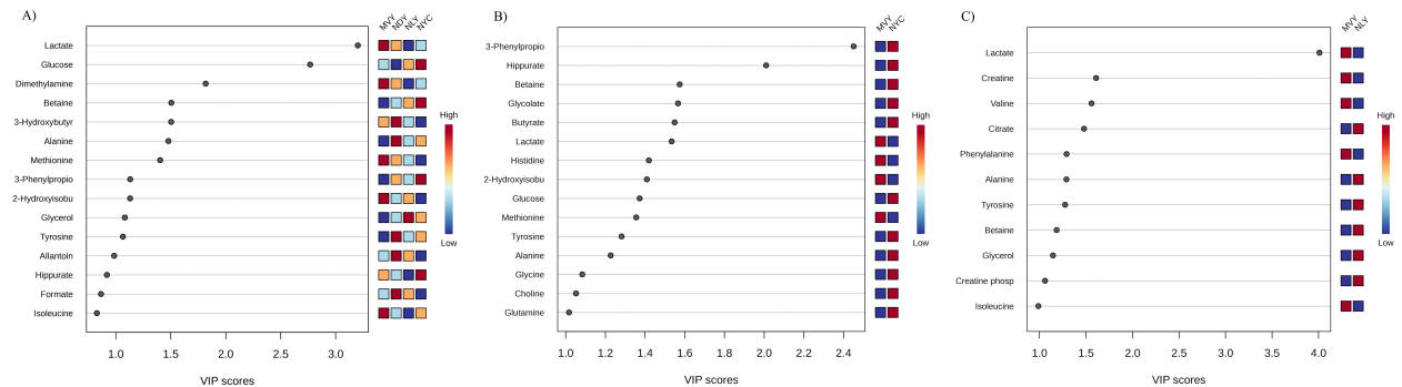
FIGURE 2 Variable importance in the projection (VIP) analysis ranking the top metabolites whose relative serum levels differ between treatment groups. (A) monensin + virginiamycin + live yeast (MVY), narasin + active dry yeast (NDY), narasin + live yeast (NLY), narasin + yeast culture (NYC) ( R^2 = 0.99 and Accuracy = 0.28); (B) monensin + virginiamycin + live yeast (MVY), narasin + yeast culture (NYC) ( R^2 = 0.91 and Accuracy = 0.66); (C) monensin + virginiamycin + live yeast (MVY), narasin + live yeast (NLY) ( R^2 = 0.94 and Accuracy = 0.55).
