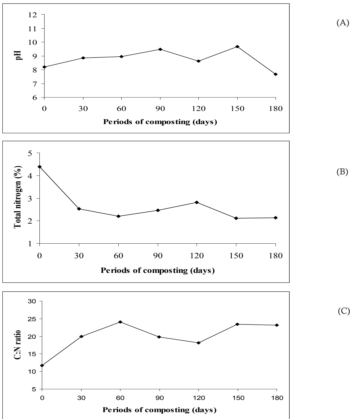
Figure 4. pH (A), total nitrogen (B) and carbon:nitrogen ratio (C) of a mixture of inedible poultry cuts and poultry litter (Capão do Leão, RS, 2007).
