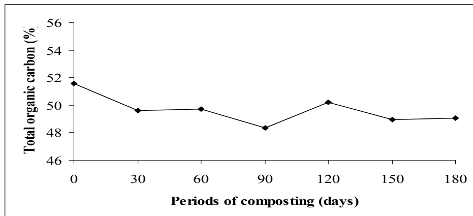
Figure 3. Moisture (A), total organic matter (B) and total organic carbon (C) of a mixture of inedible poultry cuts and poultry litter (Capão do Leão, RS, 2007).
