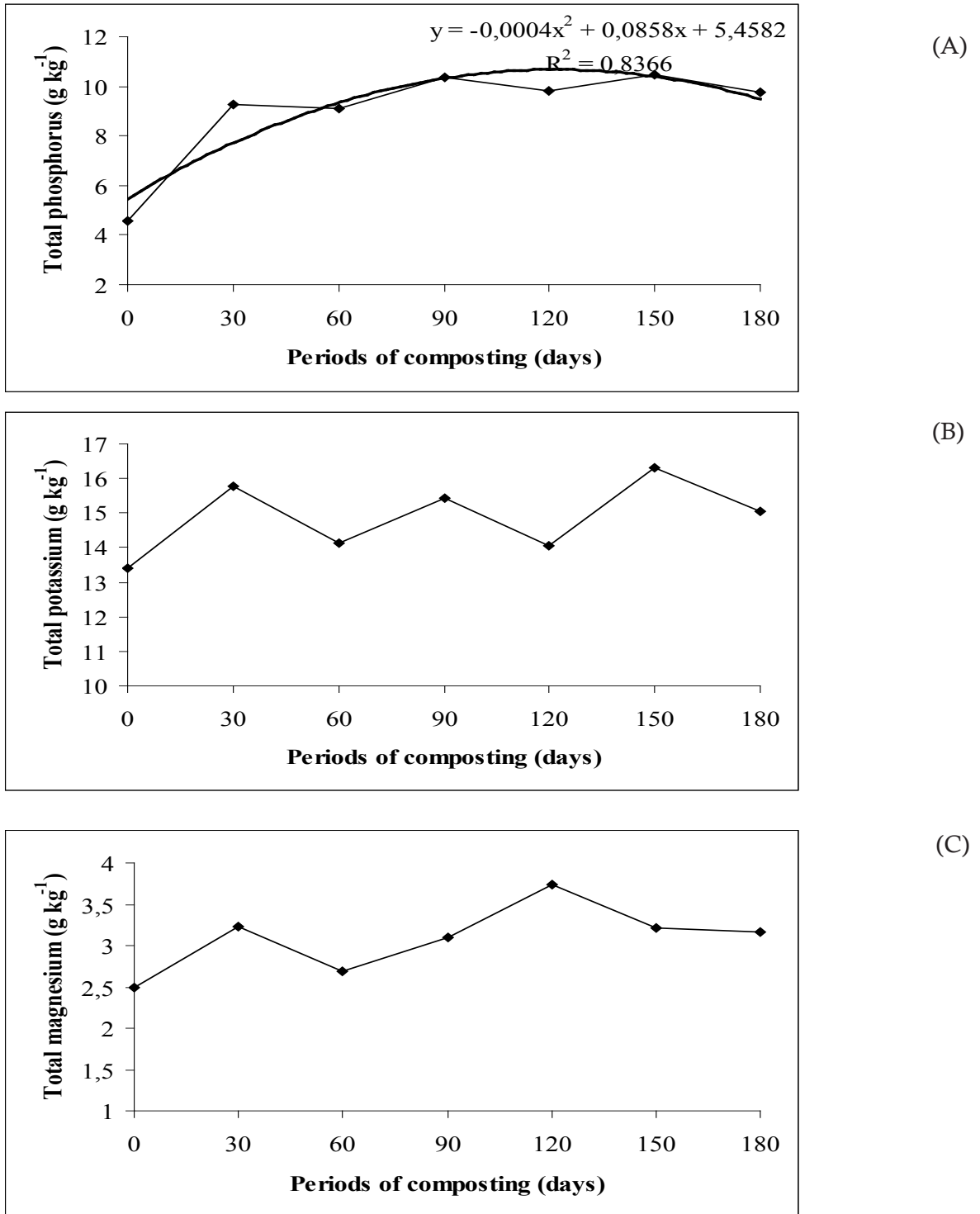
Figure 5. Total phosphorus (A), total potassium (B) and total magnesium (C) of a mixture of poultry cuts and poultry litter (Capão do Leão, RS, 2007).
