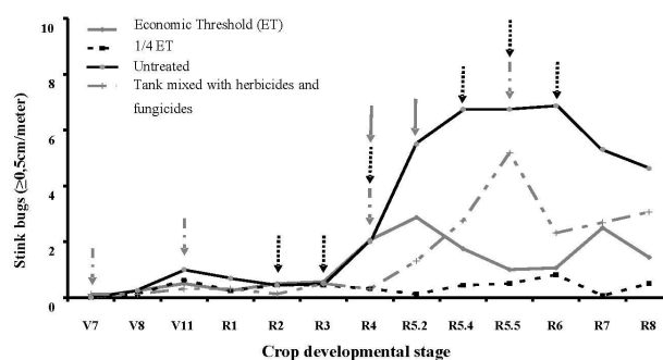
Figure 5. Mean population ( \pm SE) of stink bugs along the soybean crop developmental stages after different treatments (indicated by the arrows) for pest control. County of Arapongas, State of Paraná, Southern Brazil, 2010/2011 crop season (Bueno et al., 2013)
