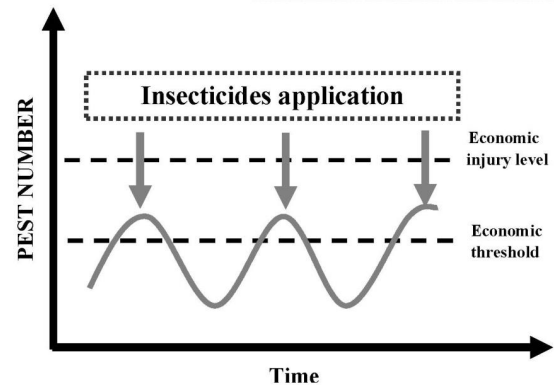
Figure 3. Graphic representation of the moment in which pest control measures have to be adopted on the soybean field according to Integrated Pest Management (IPM) recommendations
