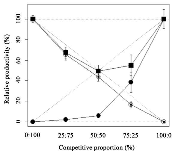
Figure 4. Relative productivity (PR) for shoot dry mass of sourgrass (●) and soybean (O), and total relative productivity (PRT) of the community (■) as a function of plant proportion (sourgrass: soybean). Dashed lines represent the expected values, in absence of competition, and solid lines the observed values when both species competed in different plant proportions. The standard error bars for treatment replications are presented for each treatment mean. Embrapa Western Agriculture, Dourados-MS, Brazil, 2015.
