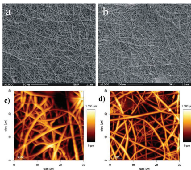
Fig. 2 SEM micrographs (a, b) and AFM images (c, d) of PVA and Cm-p1–PVA fibers. (a) 10% PVA fibers with 1000 \times magnification, (b) 10% Cm-p1–PVA fibers with 1000 \times magnification, (c) 10% PVA fibers and (d) 10% Cm-p1–PVA fibers.
