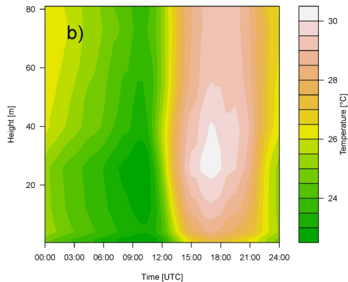
Figure 6. Diurnal profiles of temperature for (a) wet season (March 2014) and (b) dry season (September 2013). Contour plots interpolate from measurements at 0.4, 1.5, 4, 12, 26, 36, 40, 55, 73, and 81 m.
