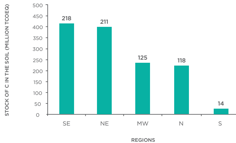
FIGURE 7. CO 2 EQ. EMISSIONS AVOIDED BY THE REGENERATION OF DEGRADED PASTURES AND BY ICLS/ICLFS BETWEEN 2012/13 AND 2022/23.
