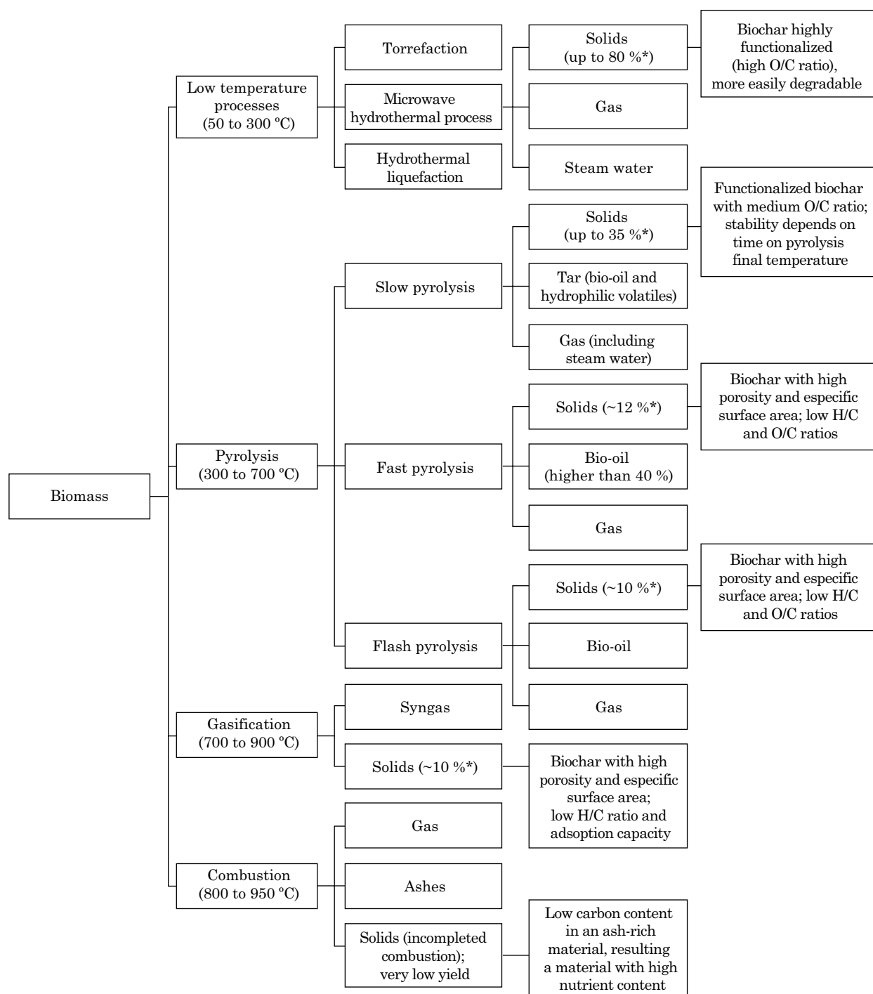
Figure 2. Thermochemical processes of biomass production, according to the temperature range and predominant biochar characteristics (*Bridgwater, 2003).
