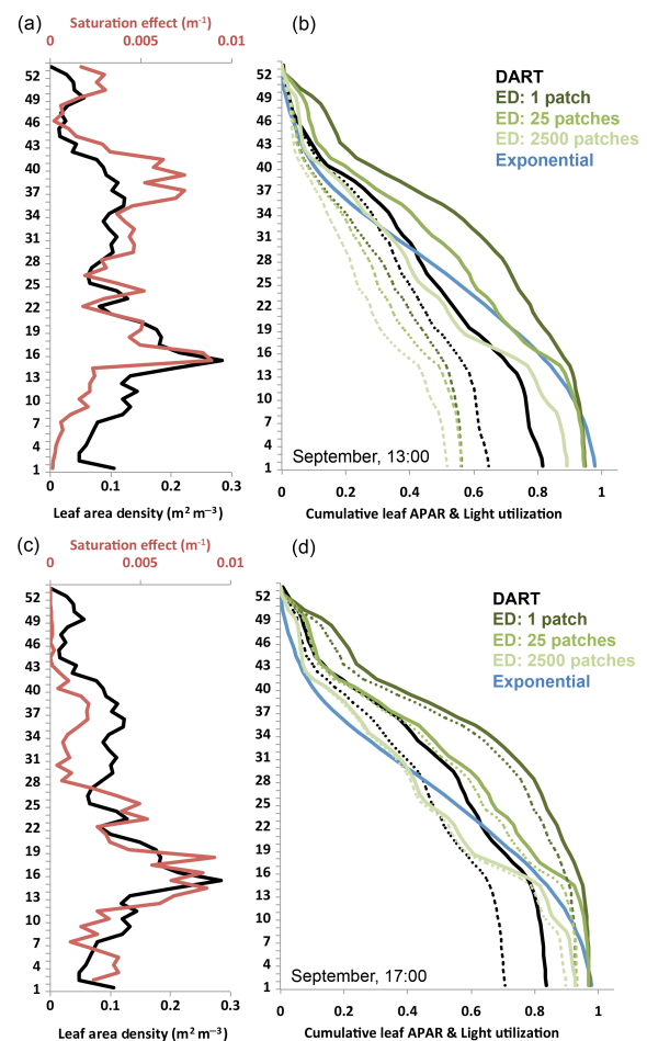
Figure 6. Forest 3-D structure alters total leaf absorption, light utilization, and the vertical distribution of light saturation effects compared to more simplified representations of the Amazon forest scene. (a) Vertical profiles of leaf area density (black) and light saturation effect (red, difference between absorbed and utilized light) for September 13:00 DART simulations. (b) DART cumulative \lambda PAR (black) and light utilization (dashed black); differences between light absorption and light utilization in DART simulations are plotted as the red curve in panel (a) to illustrate the vertical distribution of light saturation effects through the profile of canopy leaf area. DART results were compared to an exponential model of light extinction (blue, following Stark et al., 2012) and ED2 model simulations (green). Solid and dashed green lines depict cumulative leaf absorption and cumulative light utilization, respectively, for ED2 simulations with 1, 25, and 2500 patches. (c, d) Same as (a) and (b) for September 17:00 illumination conditions.
