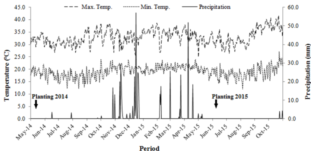
Figure 1. Rainfall (mm), maximal and minimal temperature (°C) during the trial period of 2014 and 2015 in Nova Porteirinha-MG (Source: INMET, 2015).
