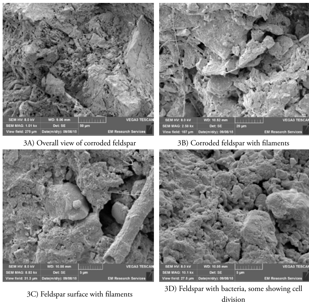
Figure 3 – Surface features of feldspar from soil developed on syenite, Triunfo, Pernambuco, Brazil.
