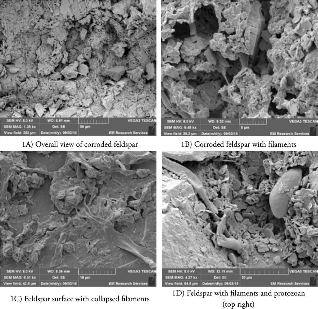
Figure 2 – Surface features of feldspar placed in soil in 2004, Eastgate, Co. Durham UK.
