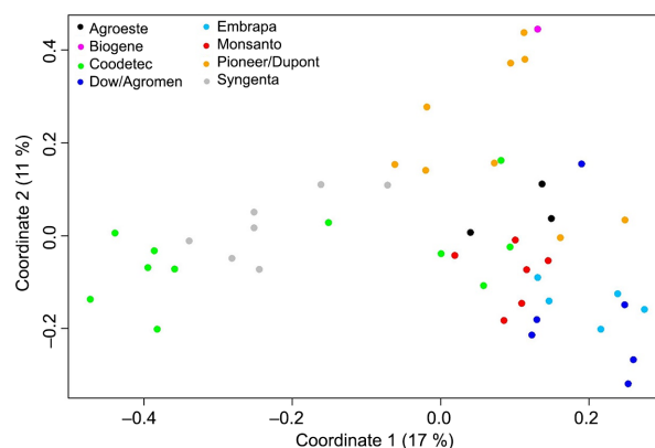
Figure 1 – Classical multidimensional scaling (MDS) biplot constructed based on 20 SSR markers obtained via the universal tail sequence primers (UTSP) method for 48 maize commercial hybrids. The percentage of variance explained by each coordinate is indicated within brackets.
