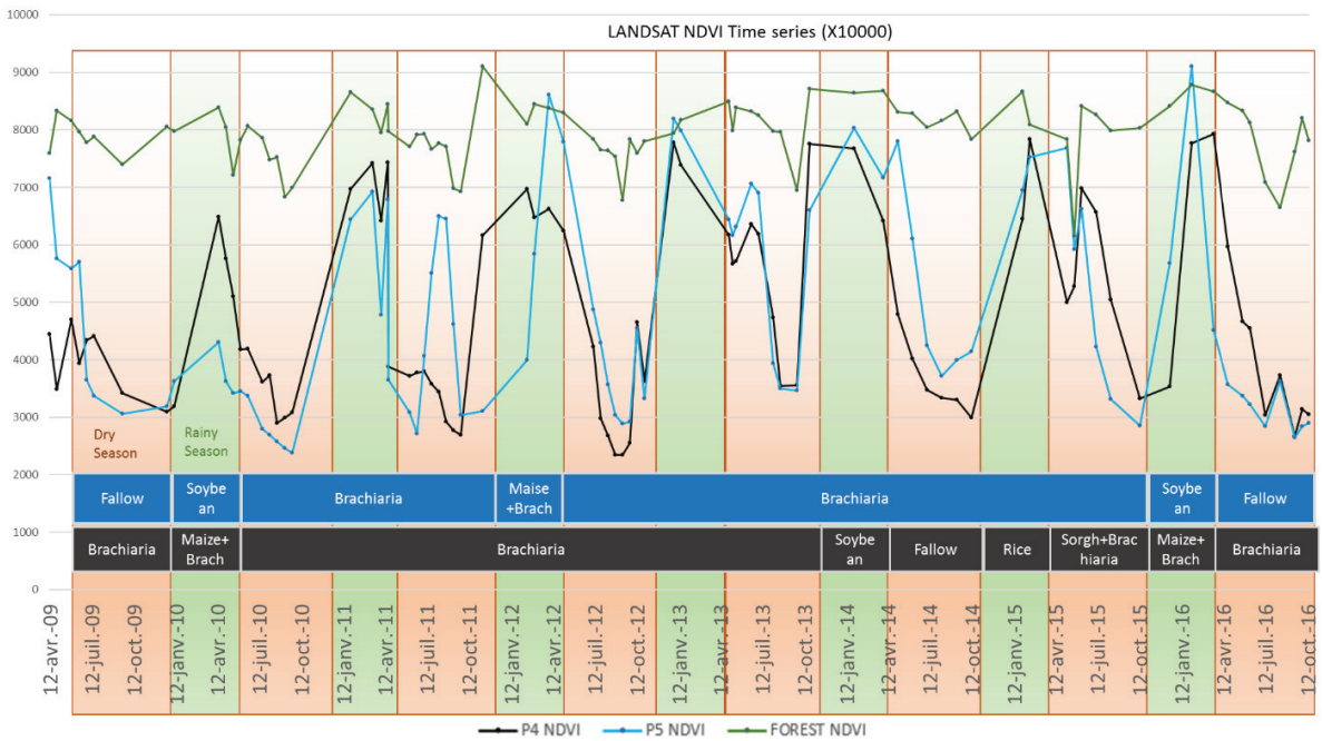
Figure 1 – Landsat NDVI time profile of different land use systems.
