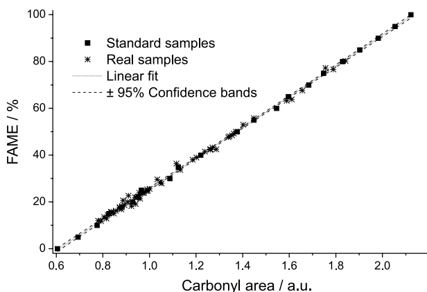
Figure 5. Calibration curve ( R^2 = 0.9994 and RMSEP = 1.1061 ) obtained with standard samples and predicted FAME concentration of real samples. The abscissa values are the integrated ester C=O stretching band.
