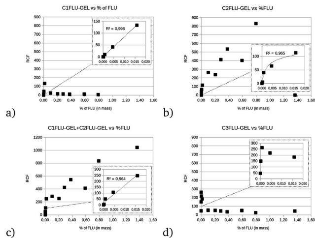
Fig. 5 CP/PARAFAC relative contribution of C_{x,FLU-GEL} versus the FLU content in the solid powder.
