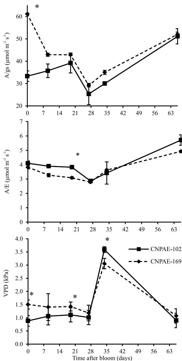
Figure 3. Evaluated parameters: A, intrinsic water-use efficiency ( A/g_s ); B, water-use efficiency ( A/E ); and C, vapor deficit pressure (VPD) of two contrasting Jatropha curcas accessions (CNPAE-102 and CNPAE-169). Bars represent the standard deviation and asterisks indicate significant differences between the means, in each evaluation time, according to the t-test, at 5% probability.
