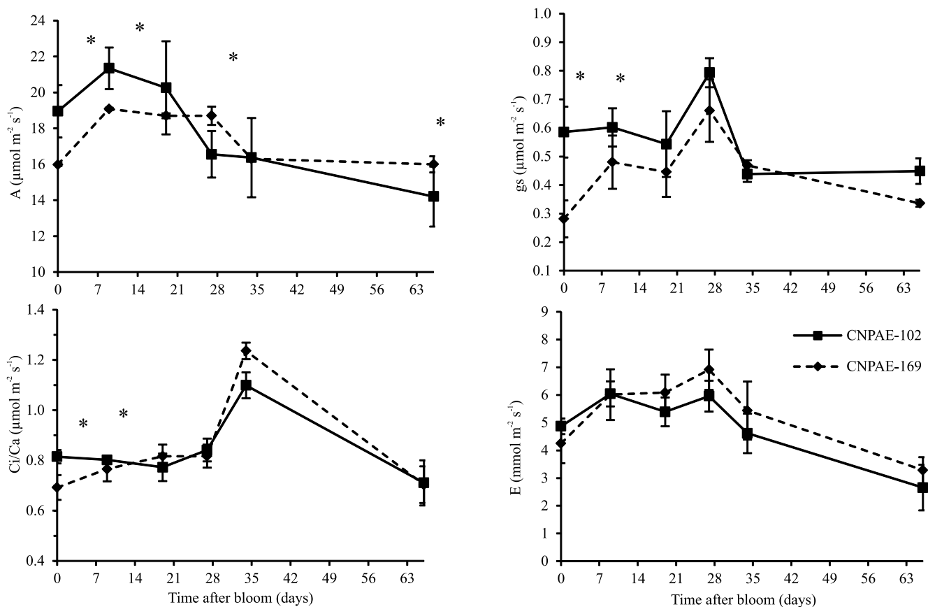
Figure 2. Evaluated parameters: A, net carbon assimilation rate ( A ); B, stomatal conductance to water vapor ( g s ); C, internal-to-ambient CO 2 concentration ratio ( C i /C a ); and D, transpiration rate ( E ) of two contrasting Jatropha curcas accessions (CNPAE-102 and CNPAE-169). Bars represent the standard deviation, and asterisks indicate significant differences between the means, in each evaluation time, according to the t-test, at 5% probability.
