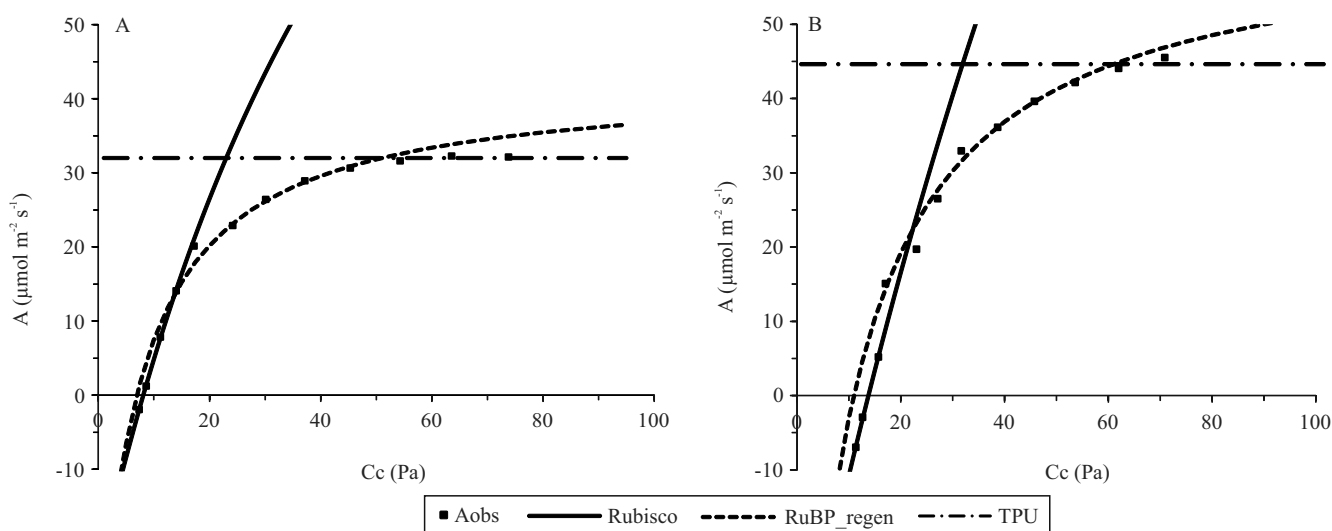
Figure 4. Response of net photosynthesis to internal leaf \text{CO}_2 concentration ( A/C_i curves) for two contrasting Jatropha curcas accessions: A, CNPAE-102; and B, CNPAE-169 during the flowering/fruiting period. Squares represent the actual measured data. Carboxylase/oxygenase (Rubisco)-limited photosynthesis stage is shown in full line, while ribulose bisphosphate (RuBP)-regeneration-limited photosynthesis stage (where A is limited by the regeneration rate of RuBP) is shown in dotted lines. Triose phosphate use (TPU) limitation stage is shown in slashed/dotted line.
