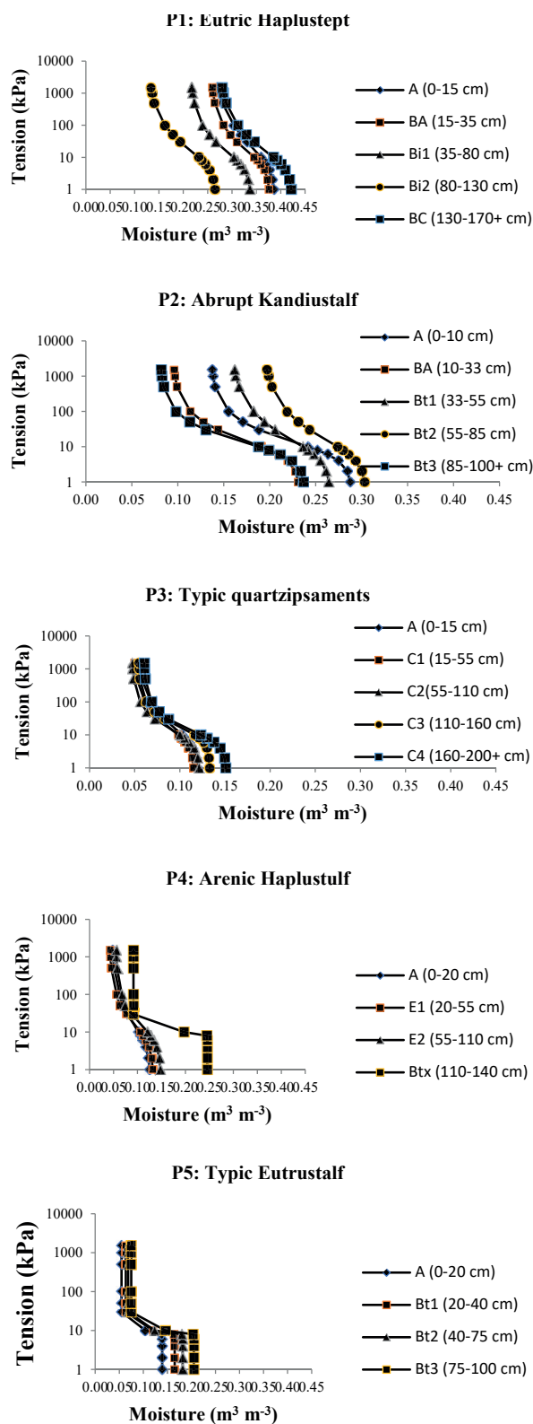
Figure 1 - Water retention characteristic curve of soils.
