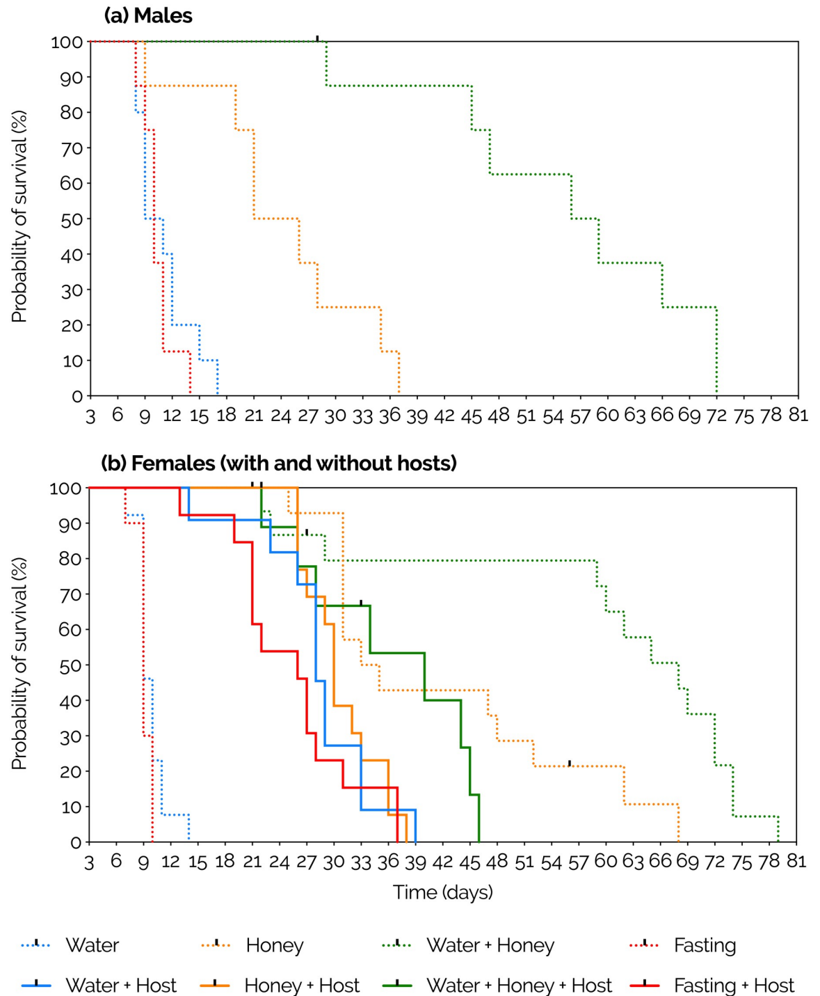
Fig 2. Effects of constant supply of water, honey, and host on the survival curves of male (a) and female (b) adults of Pachycrepoideus vindemmia (Hymenoptera: Pteromalidae) reared on pupae of spotted-wing drosophila ( Drosophila suzukii ) (Diptera: Drosophilidae). Curves were estimated according to the Kaplan-Meier method. Dark dots represent censored data (either because wasp escaped or was accidentally killed when food, water, or hosts were being replaced). Curves were compared using the log-rank (Mantel-Cox) test (details in Table 1 and S1 Table). The numbers of replicates respectively for water, honey, water + honey, and fasting (no water, no honey) were 10, 8, 9, and 8 for males; 13, 14, 16, and 10 for females; and 11, 14, 10, and 12 for host-provided females. Each replicate was formed by a mated individual wasp.
