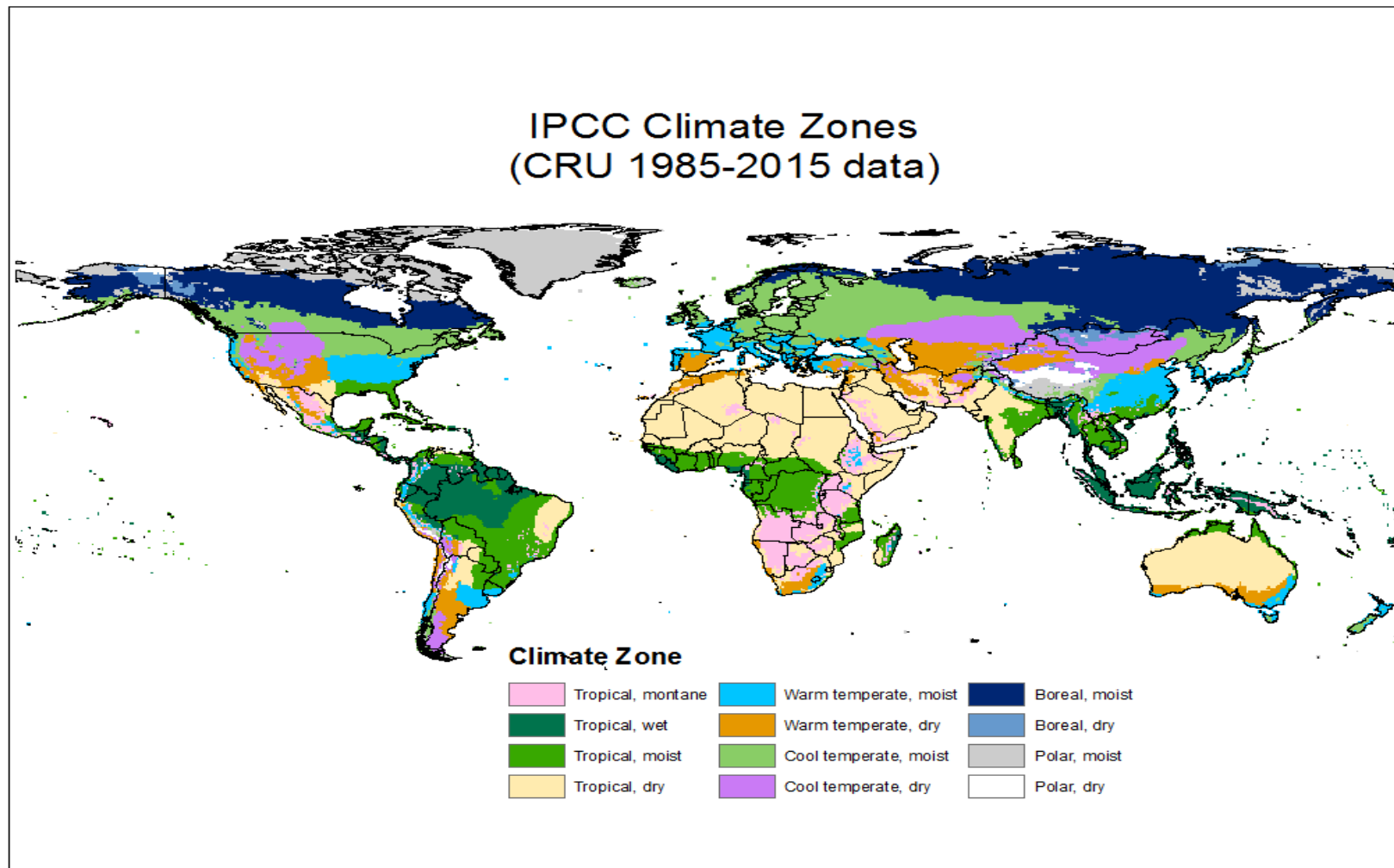
Figure 10A.1 (New) Mapping of IPCC climate zones. (taken from Volume 4, Chapter 3, Annex 3A.5)
