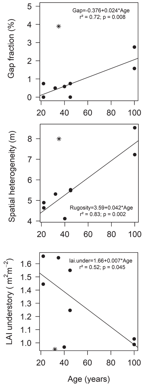
FIGURE 4 Gap fraction, canopy spatial heterogeneity, and understory leaf area index ( LAI_{\text{understory}} ) as a function of forest age. The “*” point is an outlier not included in these regressions. Old-growth forests were assigned an age of 100 years
