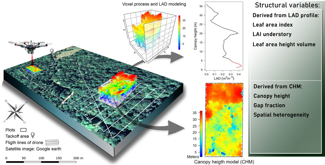
FIGURE 2 Flight plan of data collection and lidar-derived metrics. Example of a single flight in which two plots were overflowed within the maximum flight time of 15 min for the DJI Matrice 600 Pro used to transport the sensor suite
