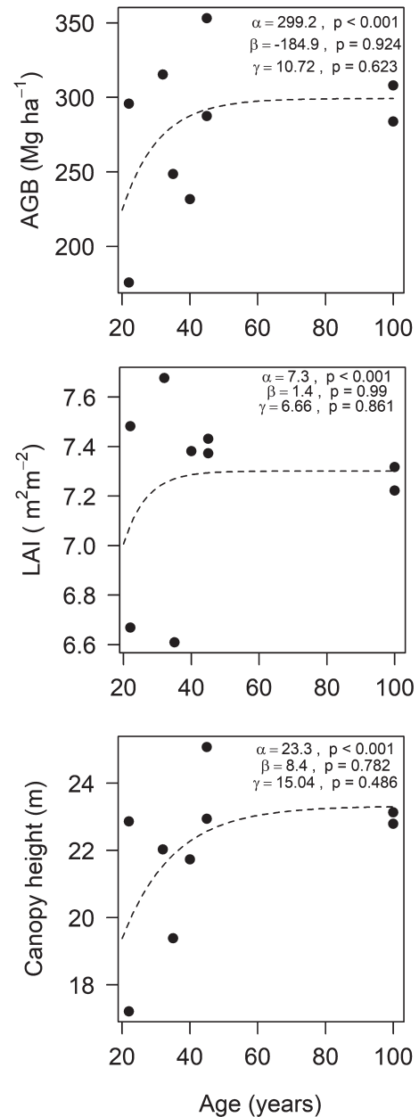
FIGURE 5 Field-derived aboveground dry wood biomass (AGB), lidar-derived canopy height, and leaf area index (LAI) as a function of forest age. The parameter \alpha is the asymptote of the model, \beta is the intercept of the model, and \gamma determines the rate of change. Old-growth forests were assigned an age of 100 years
