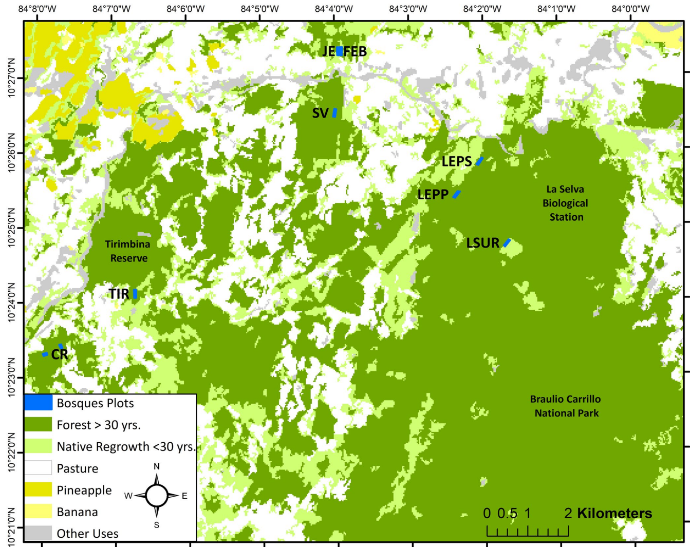
FIGURE 1 Study Area located in the Caribbean lowlands (50–220 m a.s.l.) of Heredia Province in northeastern Costa Rica. Land use classification based on satellite imagery from 2011 (Fagan et al., 2013)
