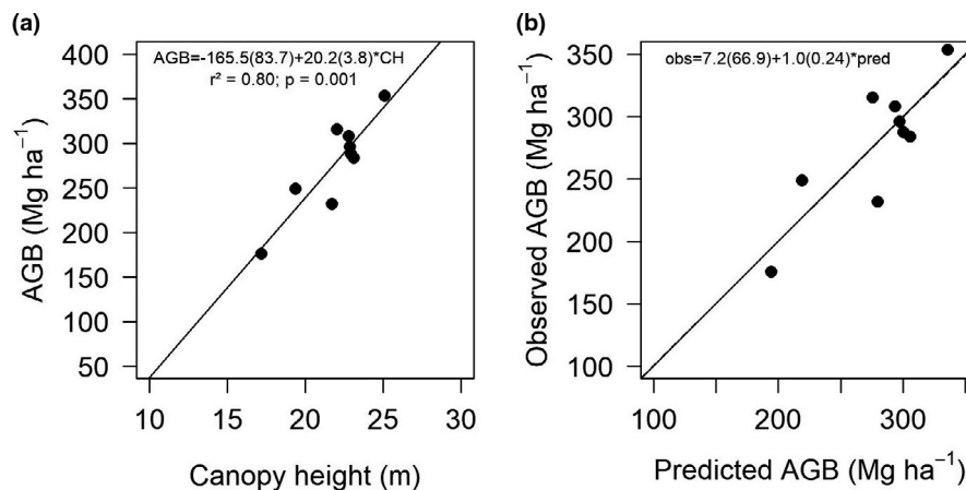
FIGURE 6 (a) Field-measured aboveground biomass (ABG) as a function of lidar-derived canopy height in nine forest plots in Sarapiquí, Costa Rica ( r^2 = .80 , p = .001 , RMSE = 24.9, relative RMSE = 9.0%). Numbers in parentheses are the standard errors for each coefficient. (b) Leave-one-out cross-validation (LOOCV) of aboveground biomass. The solid line represents a 1:1 correspondence, and the dashed line (virtually indistinguishable from the solid line) is the linear regression fit between observed and leave-one-out predicted values ( obs_i = \alpha + \beta \cdot pred_i ). The values of \alpha and \beta showed no significant difference from 0 and 1, respectively
