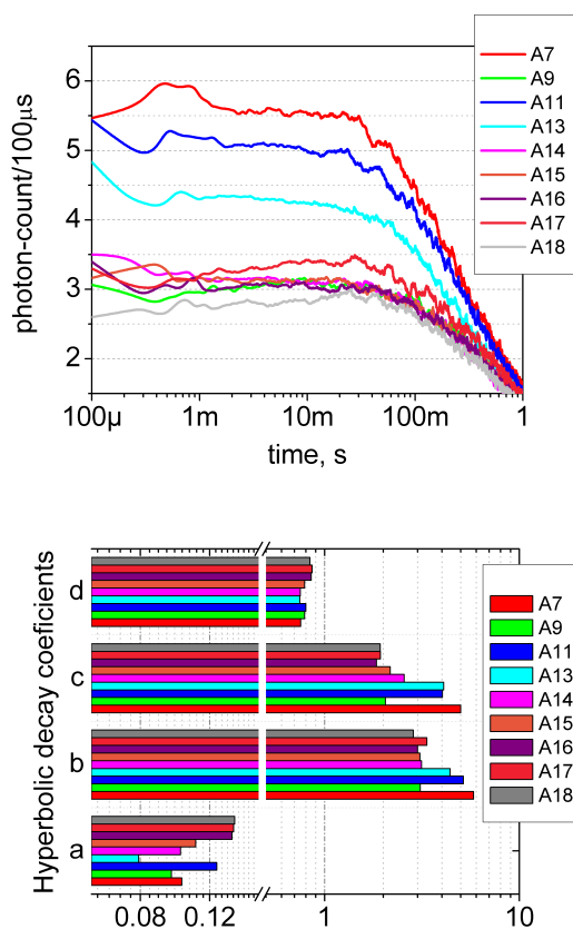
Figure 2: DL data for groups A7 to A18– (top) 10 test average time profile; (bottom) parameters of hyperbolic decay fitting ( R^2 > 0.995 ).
