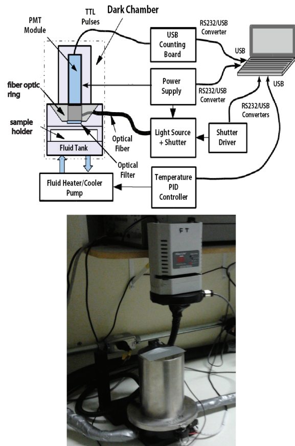
Figure 1: Setup for DL measurements in biosamples - (top) chamber, illumination and controls schematics; (bottom) picture of prototype.
