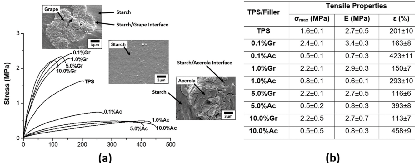
Fig. 7. Mechanical and fracture behavior. a) Stress versus strain curve and morphology for pure TPS and for biocomposites with grape skin and acerola residues. b) Tensile properties.
