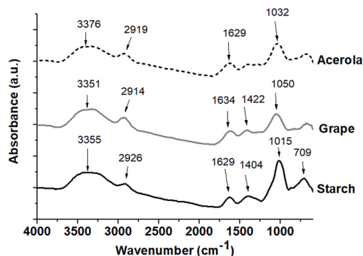
Fig. 2. FTIR spectrum of starch and grape skin and acerola residues.
