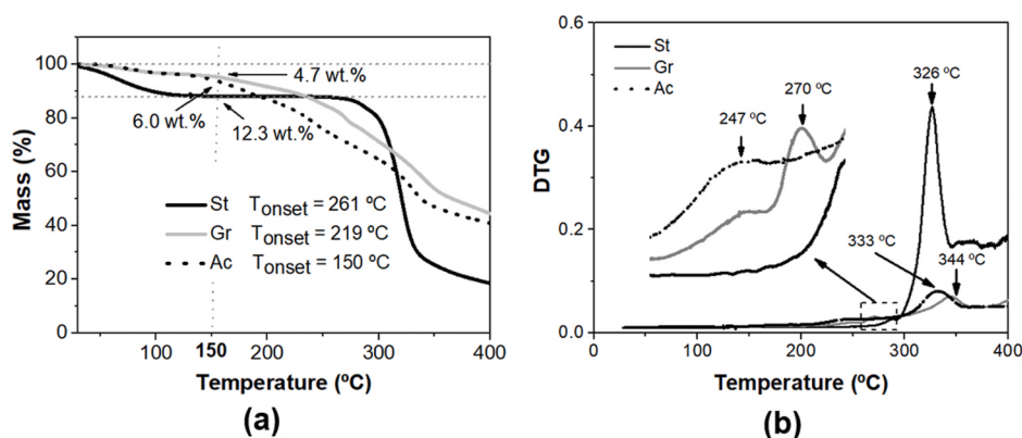
Fig. 1. Thermogravimetric curves of starch, grape skin, and acerola residues. a) TGA. b) DTG.
