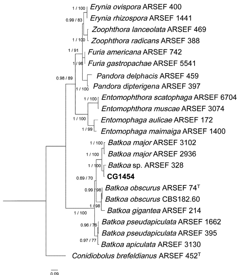
Fig. 3. Maximum likelihood phylogenetic tree generated from analysis of LSU sequence dataset for strains within the family Entomophthoraceae. Conidiobolus brefeldianus is the outgroup taxon. Support values were given as the Bayesian prior probability (first number) and percentage of bootstrap support derived from a ML analysis (second number). Ex-type strains are indicated with superscript T.
