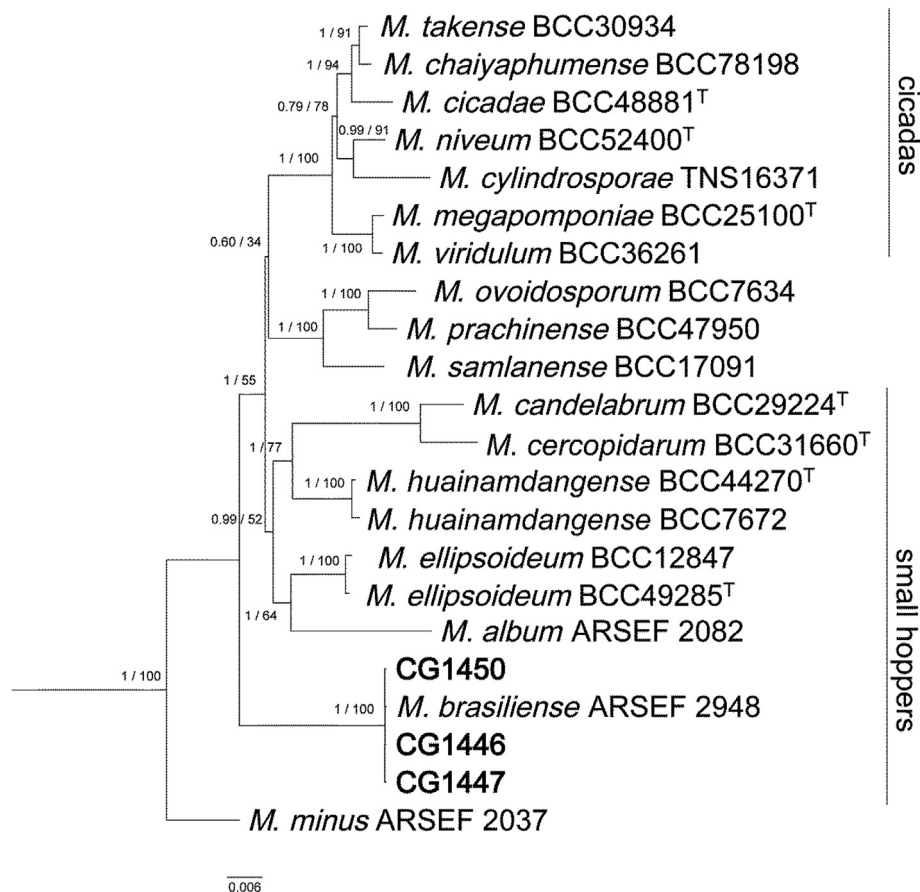
Fig. 2. Maximum likelihood phylogenetic tree generated from analyses of a combined dataset of LSU, SSU, rpb1, rpb2, and 3'tef sequences for Metarhizium strains. Metarhizium minus is the outgroup taxon. Support values were given as the Bayesian prior probability (first number) and percentage of bootstrap support derived from a ML analysis (second number). Ex-type strains are indicated with superscript T.
