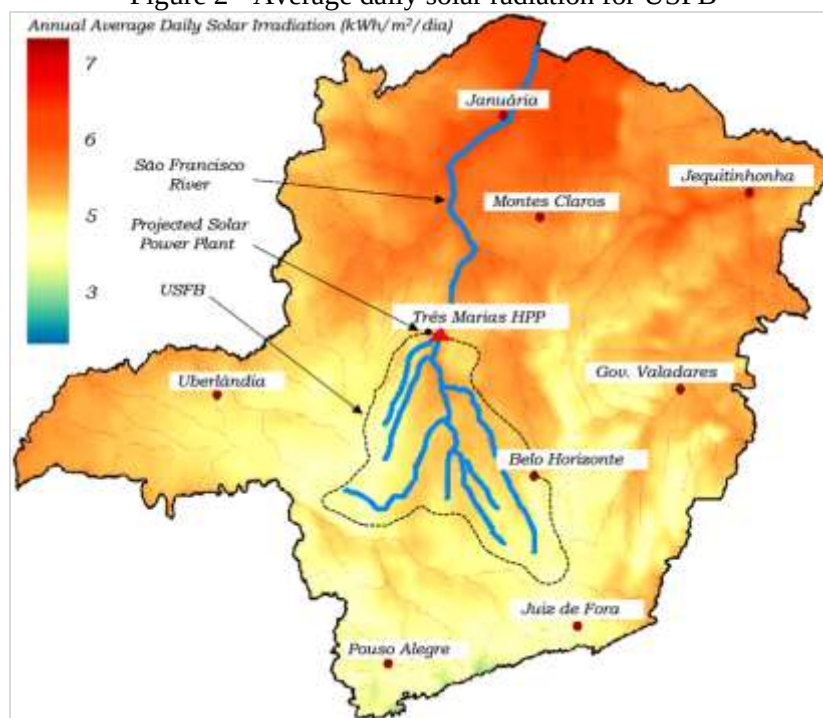
Figure 2 - Average daily solar radiation for USFB
