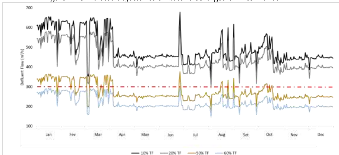
Figure 4 - Simulated trajectories of water discharged of Três Marias HPP
