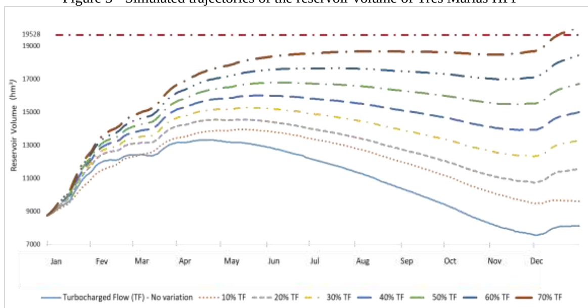
Figure 3 - Simulated trajectories of the reservoir volume of Três Marias HPP
