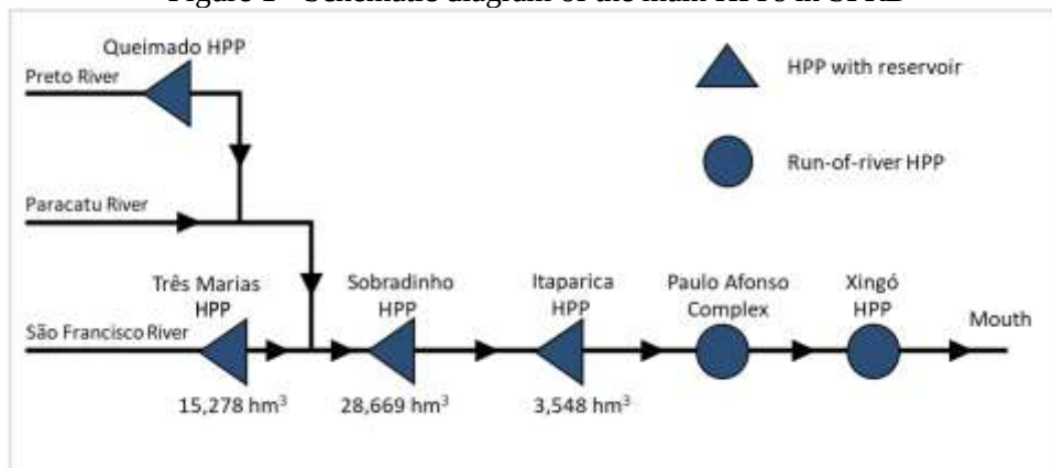
Figure 1 - Schematic diagram of the main HPPs in SFRB
