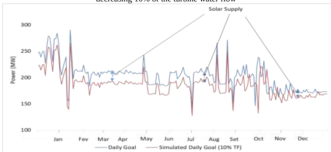
Figure 5 - In blue, energy demand, in red, energy generated by Três Marias HPP decreasing 10% of the turbine water flow
