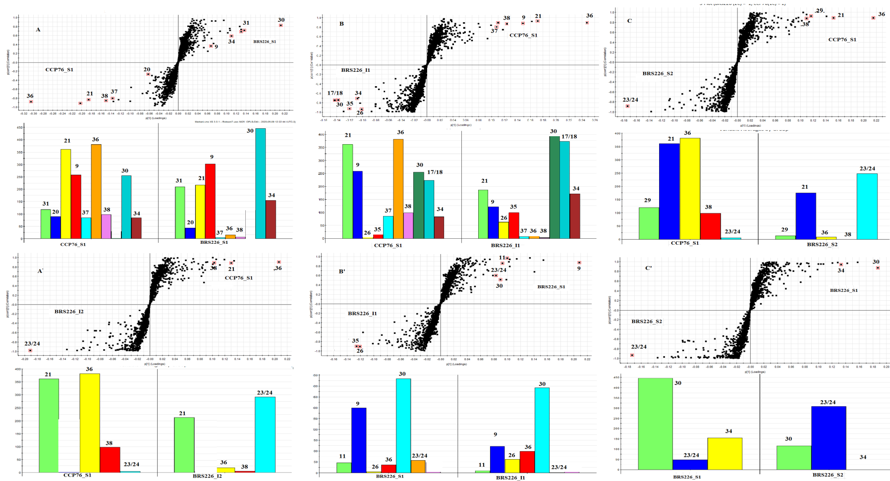
Figura 17 – Análise de S-Plot e gráficos de barras das duas variáveis de clone: (A) CCP76_S1 x BRS226_S1; (B) CCP76_S1 X BRS226_I1; (C) CCP76_S1 x BRS226_S2; (A') CCP76_S1 x BRS226_I2; (B') BRS226_S1 x BRS226_S1 e (C') BRS226_S1 x BRS226_I2.
