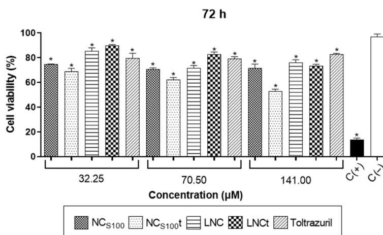
Figure 4. Cell viability of chicken fibroblasts (CEC-32 cell line) exposed to toltrazuril-loaded nanocapsules based on membrane damage (LIVE/DEAD® Viability/Cytotoxicity Kit) after (A) 24, (B) 48 and (C) 72 h. Data represent mean \pm SD ( n = 3-4 ). * p < 0.05 vs. C(-) (one-way ANOVA, post hoc Dunnett's test). NC S100 = blank Eudragit® S100 nanocapsules; NC S100t = toltrazuril-loaded Eudragit® S100 nanocapsules; LNC = blank lipid core nanocapsules; LNCt = toltrazuril-loaded lipid core nanocapsules; C(+) = positive control; C(-) = negative control. Blank formulations (NC S100 and LNC) were added the same volume, respectively, to the drug-loaded nanoformulation.
