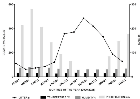
Fig. 2. Contribution of senescent litter against climatic variables (temperature, humidity and precipitation) in the period from February 2021 to January 2022 in a sedimentary basin humid forest refuge in Chapada do Araripe, Crato, Ceará, Northeastern Brazil.
