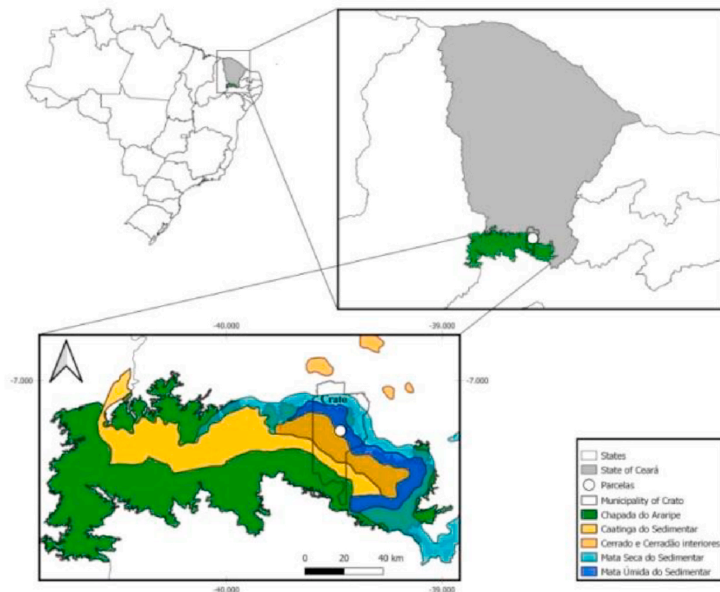
Fig. 1. Geographic location of the area of study. Sedimentary basin humid forest refuge in the Chapada do Araripe, Crato, Ceará, Northeastern Brazil.
