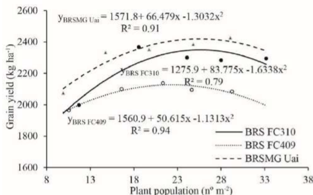
Figure 1. Grain yield of common bean cultivars BRS FC310, BRS FC409, and BRSMG Uai as a function of final plant population in experiments conducted at various sowing seasons and locations.
