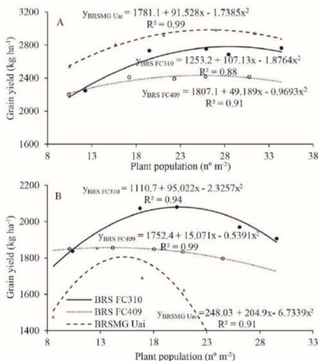
Figure 3. Grain yield of common bean cultivars BRS FC310, BRS FC409, and BRSMG Uai as a function of final plant population in experiments conducted at wet (A) and winter (B) seasons, in different locations.
