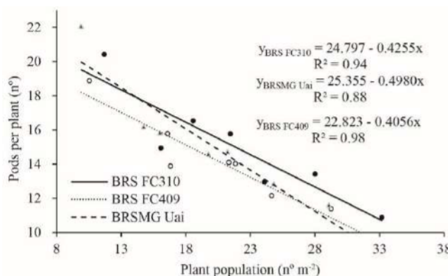
Figure 2. Pods per plant of common bean cultivars BRS FC310, BRS FC409, and BRSMG Uai as a function of final plant population in experiments conducted at various sowing seasons and locations.
