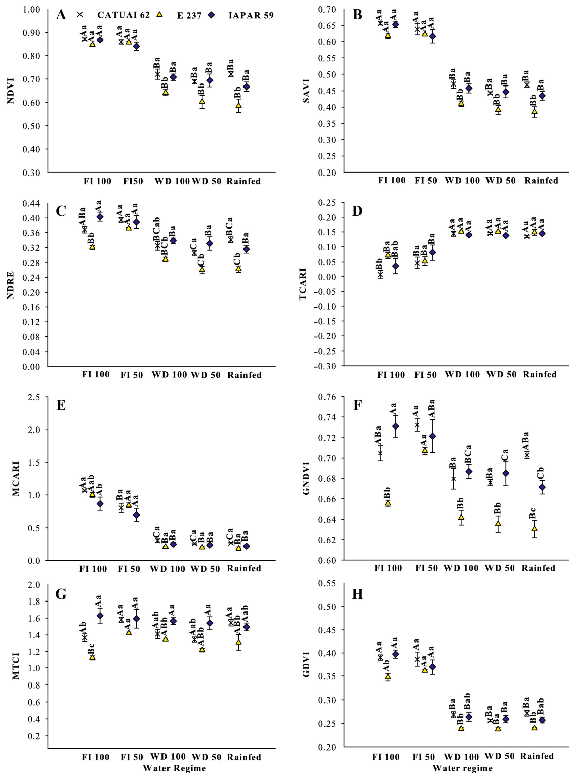
Figure 3. Vegetation indices (A) NDVI, (B) SAVI, (C) NDRE, (D) TCARI, (E) MCARI, (F) GNDVI, (G) MTCI and (H) GDVI, in 2019, for three coffee genotypes (Catuai 62, E237 and Iapar 59) under five water regimes (FI 100%, FI 50%, WS 100%, WS 50% and Rainfed) during water stress in drought treatments in 2019. Means followed by the same capital letters compare water regimes for each coffee genotype, and lowercase letters compare coffee genotypes within each water regime.
