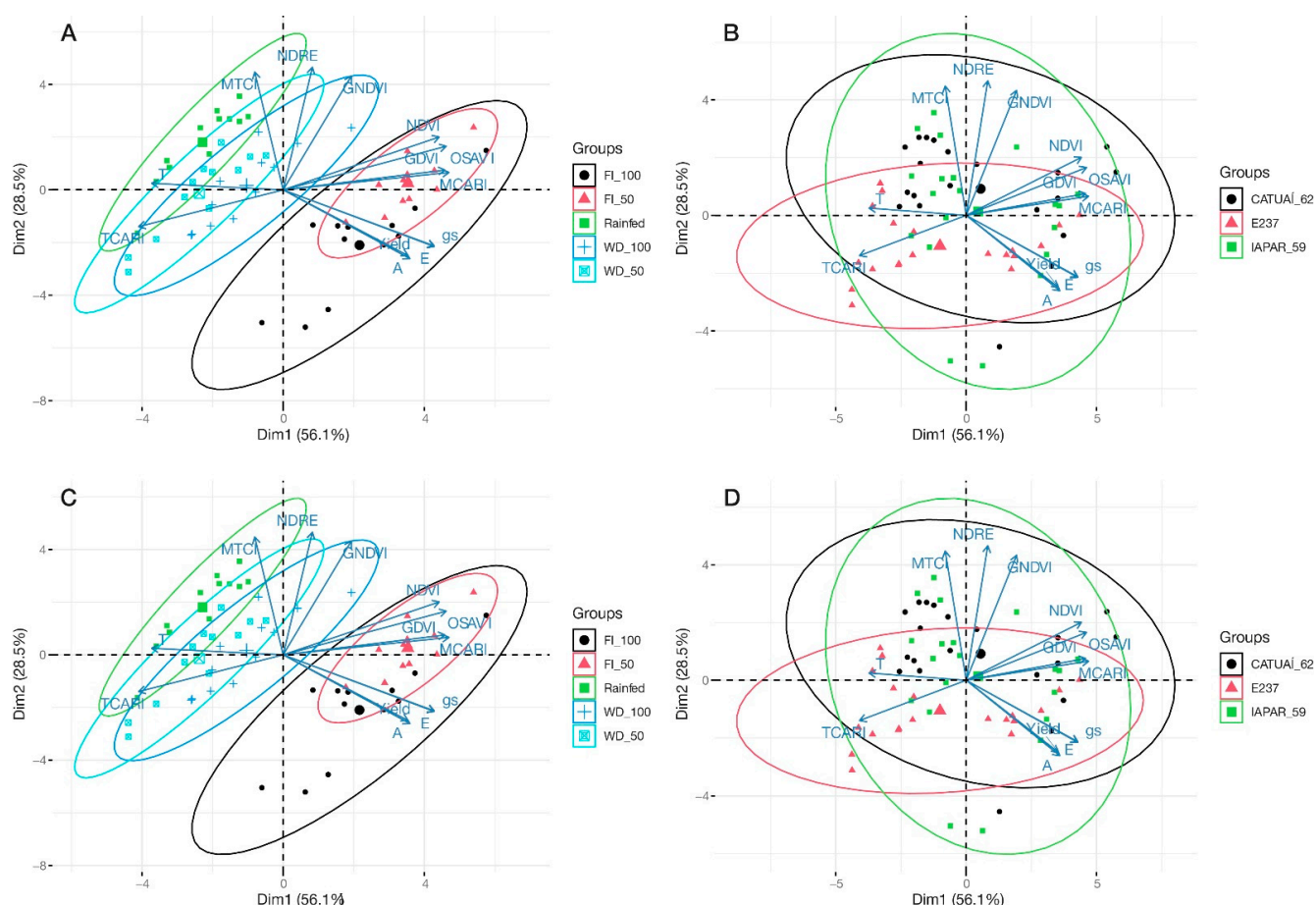
Figure 9. Exploratory analysis of the principal components for vegetation indices and coffee tree physiology and productivity in response to different water regimes and of different genotypes in the growing seasons of 2019 (A,B) and 2020 (C,D). The vectors of the variables projected onto the graphs indicate the magnitude and direction of their contribution to the separation between groups. The length of the vectors reflects the intensity of their influence on the principal components, while their orientation highlights the multivariate differences between the evaluated conditions. The ellipses drawn around the experimental groups represent the intragroup dispersion based on the covariance of the data. The center of each ellipse corresponds to the centroid of the respective group, representing the average position of the observations. The orientation and size of the ellipses indicate the internal variability of each group: more compact ellipses suggest greater homogeneity within the observations. In contrast, larger ellipses indicate greater heterogeneity, possibly associated with the different conditions imposed by the treatments. The distribution of the vectors and the separation of the ellipses demonstrate that the analyzed variables play a significant role in differentiating between the groups of cultivars and irrigation regimes, providing insights into the physiological and spectral responses under each evaluated scenario.
