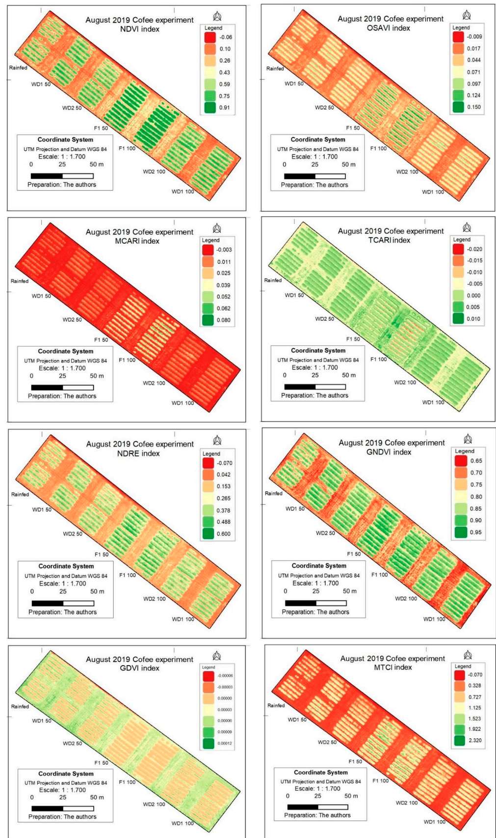
Figure 5. Vegetation indices NDVI, OSAVI, MCARI, TCARI, NDRE, GNDVI, GDVI and MTCI evaluated for three coffee genotypes (Catuaí 62, E237 and Iapar 59) in response to five water regimes (from left to right, rainfed; WD1 (water stress) 1, 50%; WD2 50%; F1 (full irrigation) 50%; F1 100%) in 2019.
