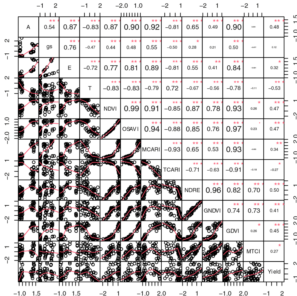
Figure 7. Correlogram of Pearson's correlation between vegetation indices and leaf gas exchange in 2019. A: photosynthesis, gs: stomatal conductance, E: transpiration and canopy temperature °C. Values close to 1 indicate a strong positive correlation, while values close to -1 represent a strong negative correlation. Values close to 0 suggest an absence of significant linear relationship. In addition, the size of the source observed in the correlogram was used to graphically represent the magnitude of the correlation, allowing a clear visualization of the strength of the associations. Stronger correlations (positive or negative) were highlighted with larger font size and bold, while weaker correlations were presented with smaller and unbold fonts. The statistical significance of the correlations was evaluated at a probability level: * significant at p < 0.05 , ** significant at p < 0.01 , *** significant at p < 0.001 .
