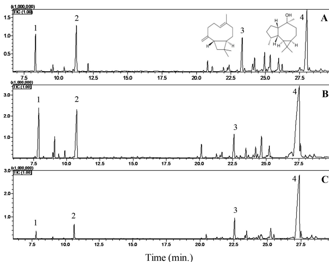
Figure 1. Chromatographic profile of essential oils of Varronia curassavica . A: parental accession VCUR-503; B: VCUR-503-101, and C: VCUR-503-119. Major peaks – 1: \alpha -pinene, 2: \beta -phellandrene, 3: E -caryophyllene, and 4: viridiflorol. Structure of the compounds E -caryophyllene and viridiflorol.
