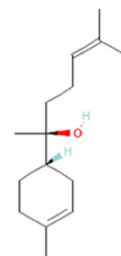
(-)\text{-}\alpha\text{-bisabolol}
