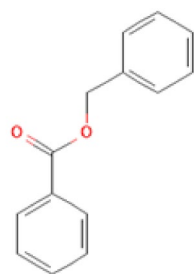
Benzyl benzoate
