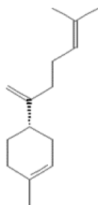
\beta -bisabolene
