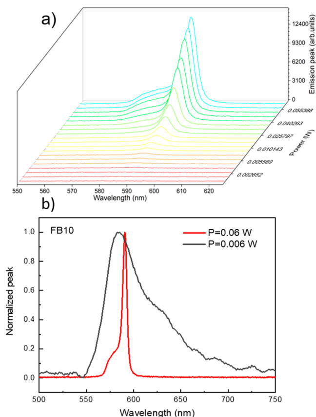
Figure 3. (a) Emission spectra as a function of pump power for FB10. (b) Emission spectrum for the sample FB10. The black line represents the emission spectrum under low excitation power (fluorescence/spontaneous emission regime), while the red line corresponds to the emission spectrum when the platform is excited with powers exceeding the laser threshold (laser regime).
