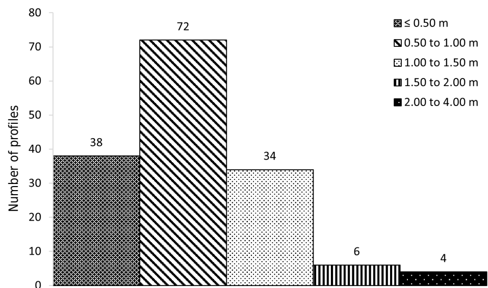
Figura 2. Profiles distribution by initial depths of the spodic B horizons of Espodossolos classified according to the original database and SiBCS (Santos et al., 2018).
