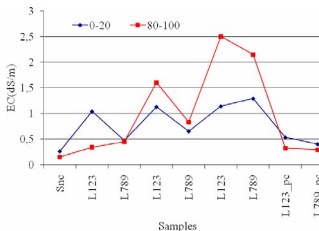
Fig. 1. Variation of the electrical conductivity (CE) of the saturation extract for cultivated and non-cultivated soil (CESnc) at 0-20 and 80-100cm soil profile, throughout the productivity cycle of the grapevine. Petrolina-PE.
