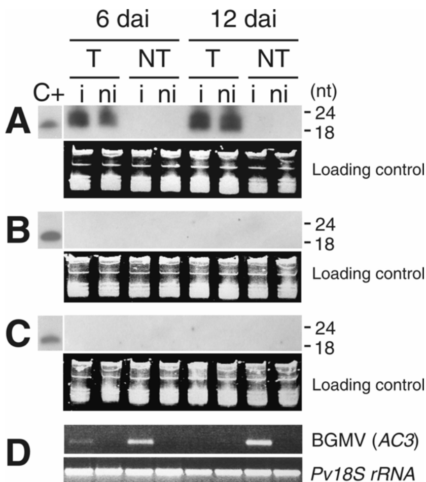
Fig. 5. Northern blot analysis of small interfering (si)RNA isolated from intron-hairpin RNA-transformed common bean plants. Plants were maintained in contact with viruliferous whiteflies for a period of 6 days. RNA was isolated from the primary leaves at days 6 and 12 from transgenic (T) and nontransgenic (NT) plants, inoculated (i) and noninoculated (ni) with Bean golden mosaic virus (BGMV). RNA blots were probed to detect the presence of siRNA molecules corresponding to A , AC1 , B , AC2 , and C , AC3 mRNA sequences. C+: 50 ng of a BGMV AC1 (in A), AC2 (in B), and AC3 (in C) gene-derived oligomers. Ethidium bromide-stained RNA serves as the loading control. All transgenic plants remained free of symptoms, whereas all nontransgenic plants had severe symptoms. D , The virus DNA was detected in a semiquantitative polymerase chain reaction. The genomic Pv18S rRNA gene was used as internal control.
