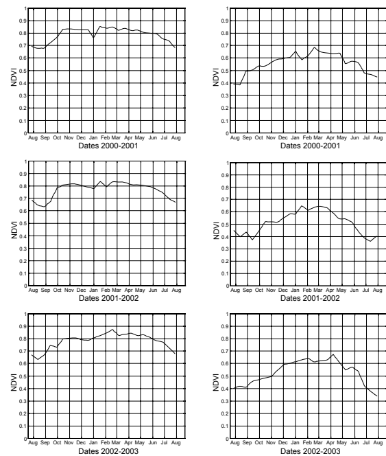
Fig. 5 - NDVI temporal profiles for areas of LULC classes savannah (left column) and pasture (right column), for years 2000-2001 (first line), 2001-2002 (second line) and 2002-2003 (third line). Overall response patterns can be seen to remain stable over the years. However, since the two class profiles differ very little in shape, class discrimination must rely almost exclusively on occasionally subtle differences in absolute NDVI values.
