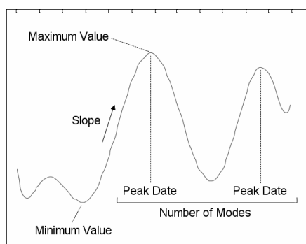
Fig. 2 - Examples of profile features computed for a MODIS NDVI temporal profile, which provide more meaningful and compact information about the temporal behavior observed at each point.
