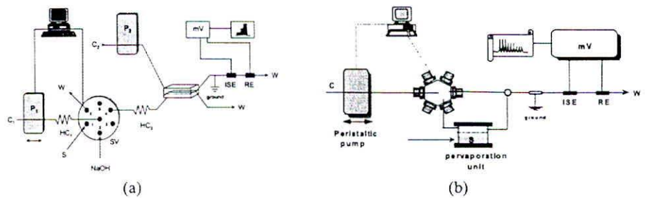
Figure 1 - Sequential injection system developed for volatile nitrogen determination. (a) Silage samples: S, sample (150 ml); NaOH, alkaline solution 3.0 mol l -1 (300 ml); HC 1 and HC 2 , holding coil (3 ml and 50 cm, respectively); C 1 and C 2 , carrier streams (H 2 O and TRIS-HCl buffer solution 0,01 mol l -1 ); ISE, ion selective electrode; RE; reference electrode; P1 and P2, peristaltic pumps and W, waste. (b) Soil samples.
