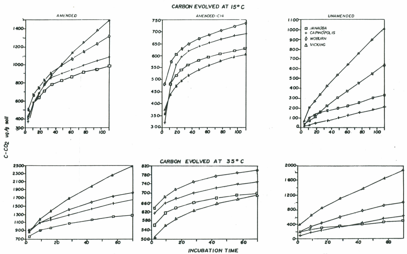
FIG. 1. Cumulative mineralization of C during incubation at 15°C and 35°C, amended and unamended with C 14 -glucose.
