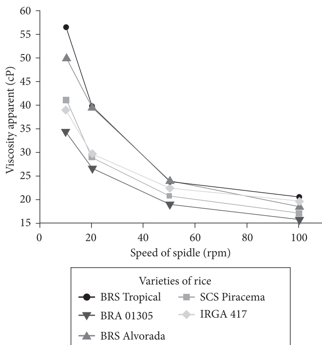
Figure 2. Apparent viscosity behavior of rice grains from the irrigated cropping system.
