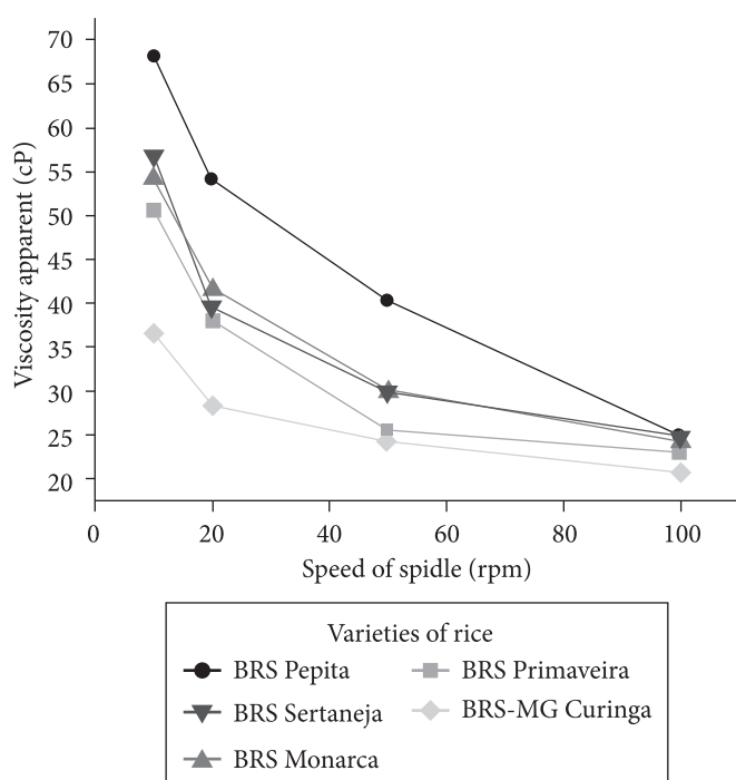
Figure 1. Apparent viscosity behavior of rice grains from the upland cropping system.
